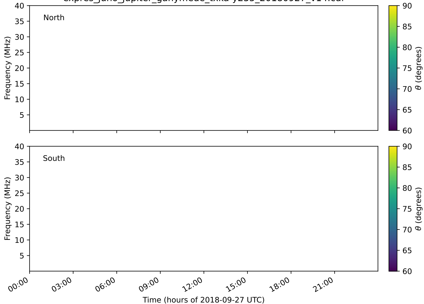
expres_juno_jupiter_ganymede_txka-y235_20180927_v14.cdf
