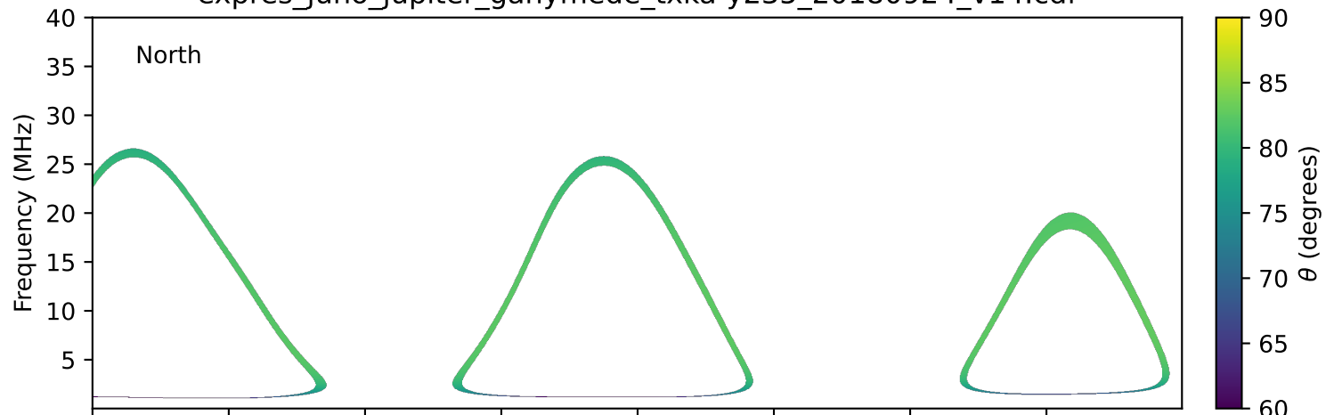
expres_juno_jupiter_ganymede_txka-y235_20180924_v14.cdf
