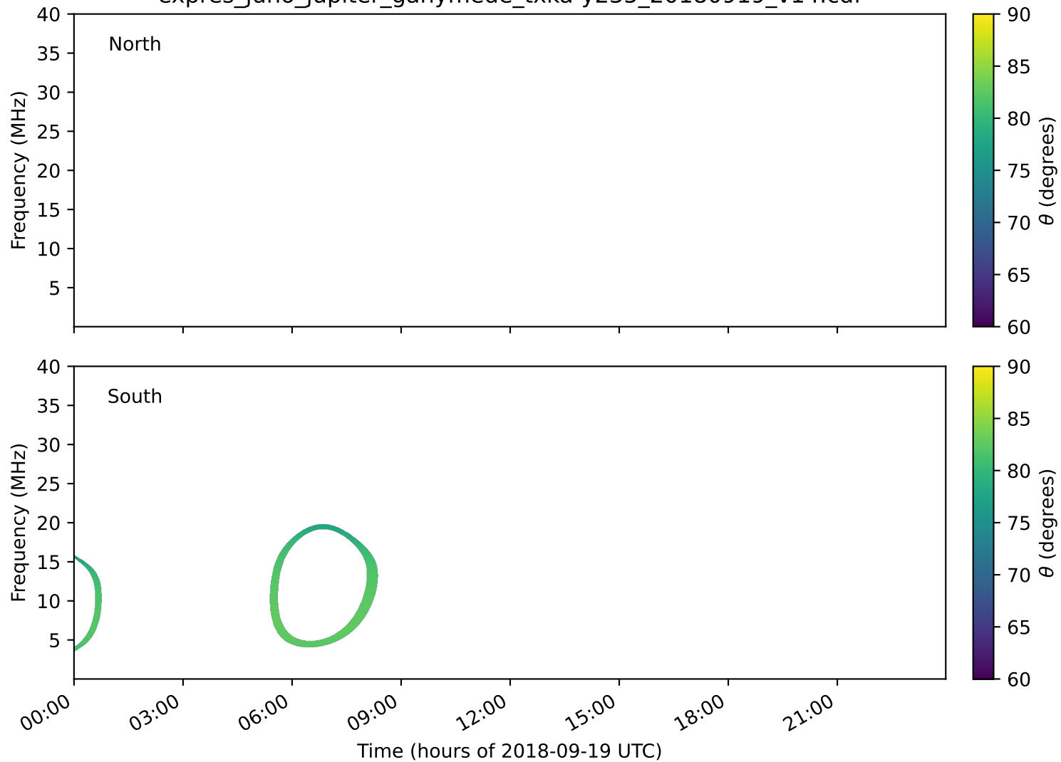
expres_juno_jupiter_ganymede_txka-y235_20180919_v14.cdf
