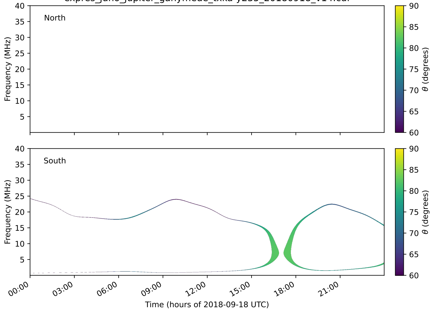
expres_juno_jupiter_ganymede_txka-y235_20180918_v14.cdf
