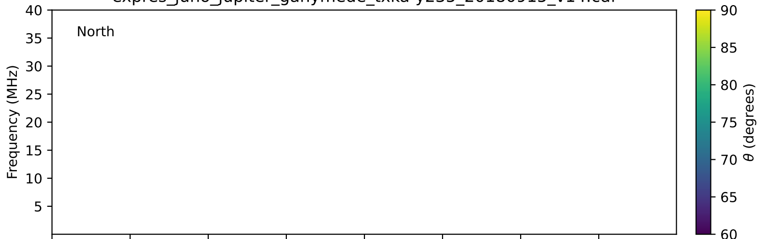
expres_juno_jupiter_ganymede_txka-y235_20180915_v14.cdf
