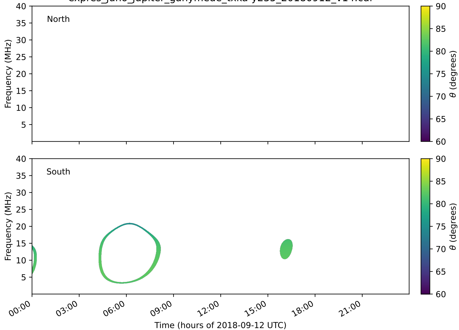
expres_juno_jupiter_ganymede_txka-y235_20180912_v14.cdf
