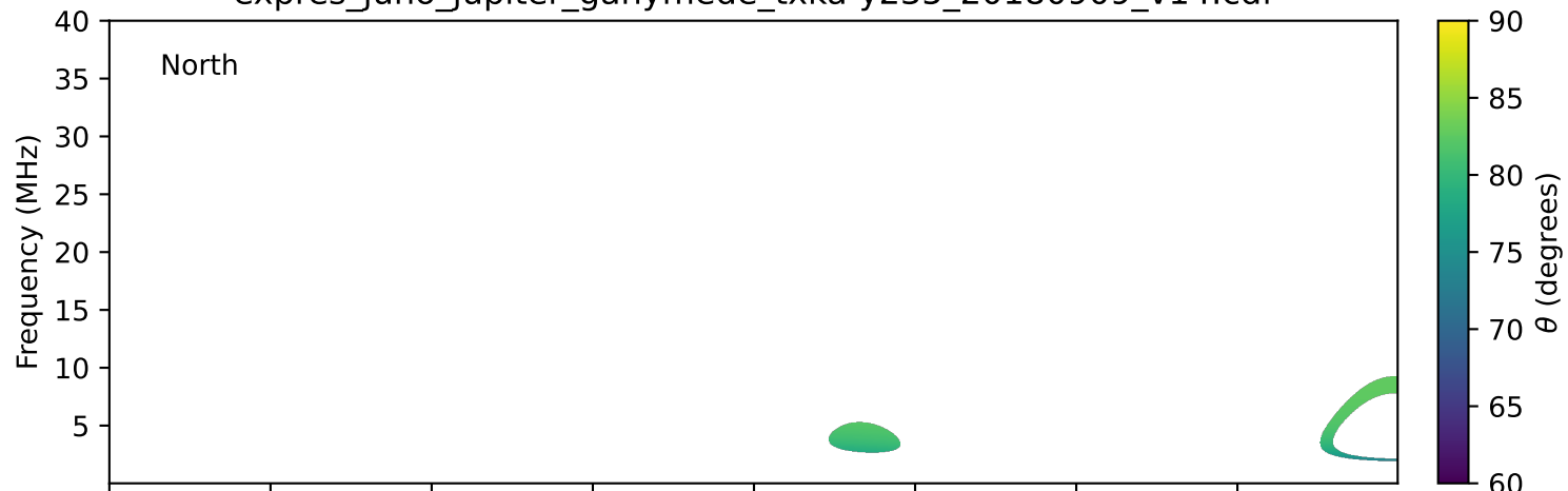
expres_juno_jupiter_ganymede_txka-y235_20180909_v14.cdf
