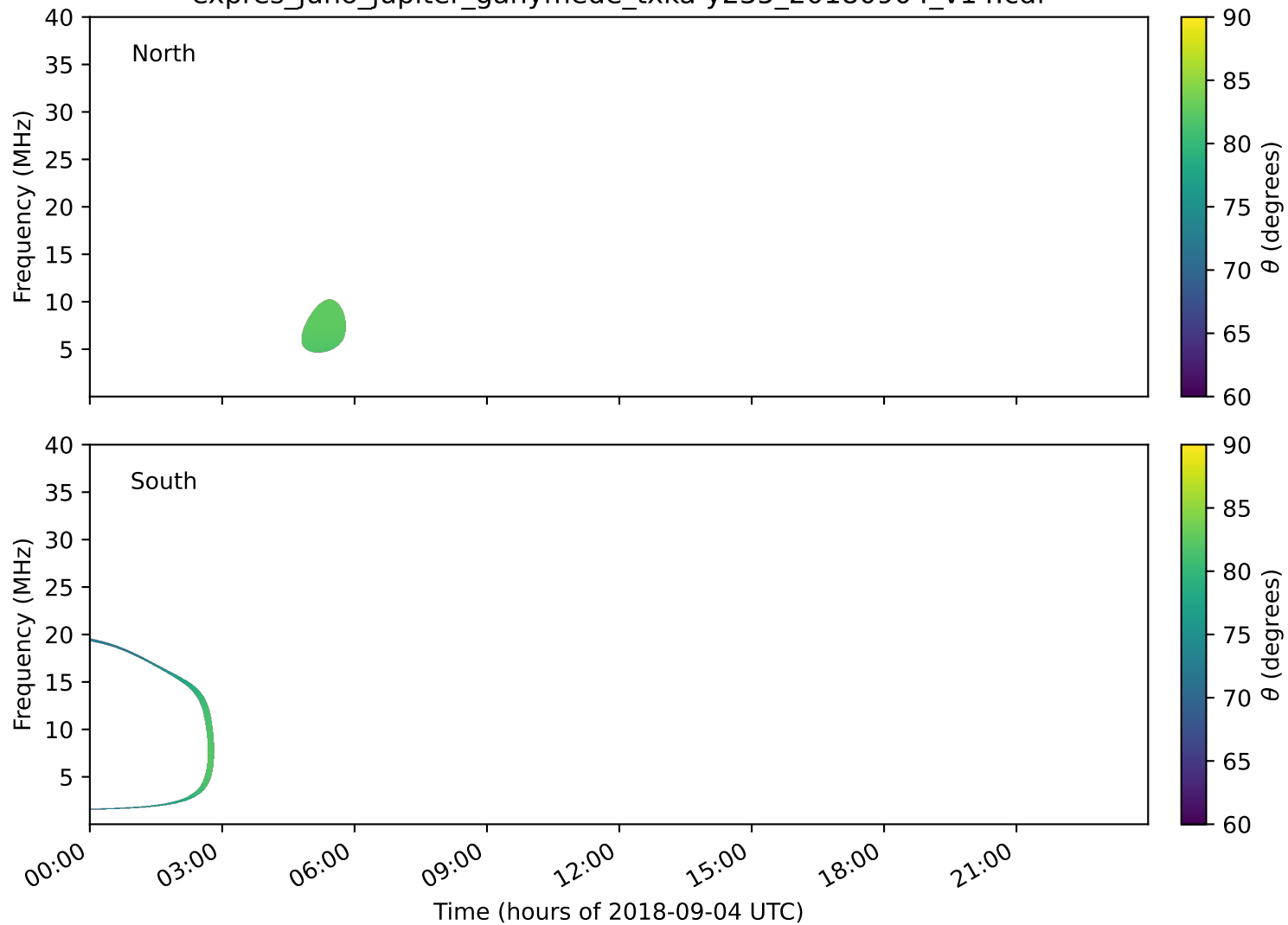
expres_juno_jupiter_ganymede_txka-y235_20180904_v14.cdf
