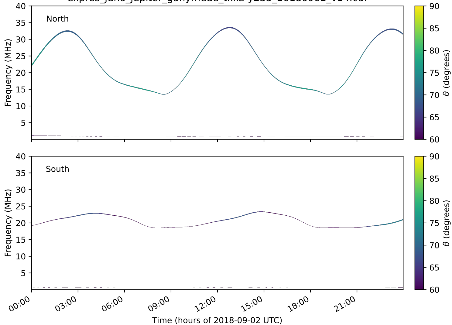
expres_juno_jupiter_ganymede_txka-y235_20180902_v14.cdf
