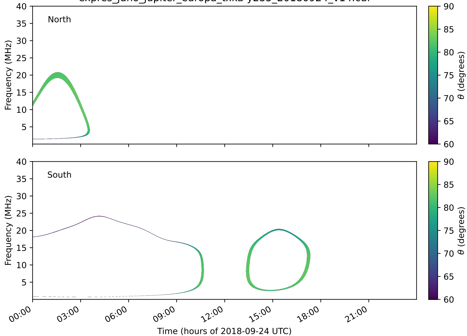
expres_juno_jupiter_europa_txka-y235_20180924_v14.cdf
