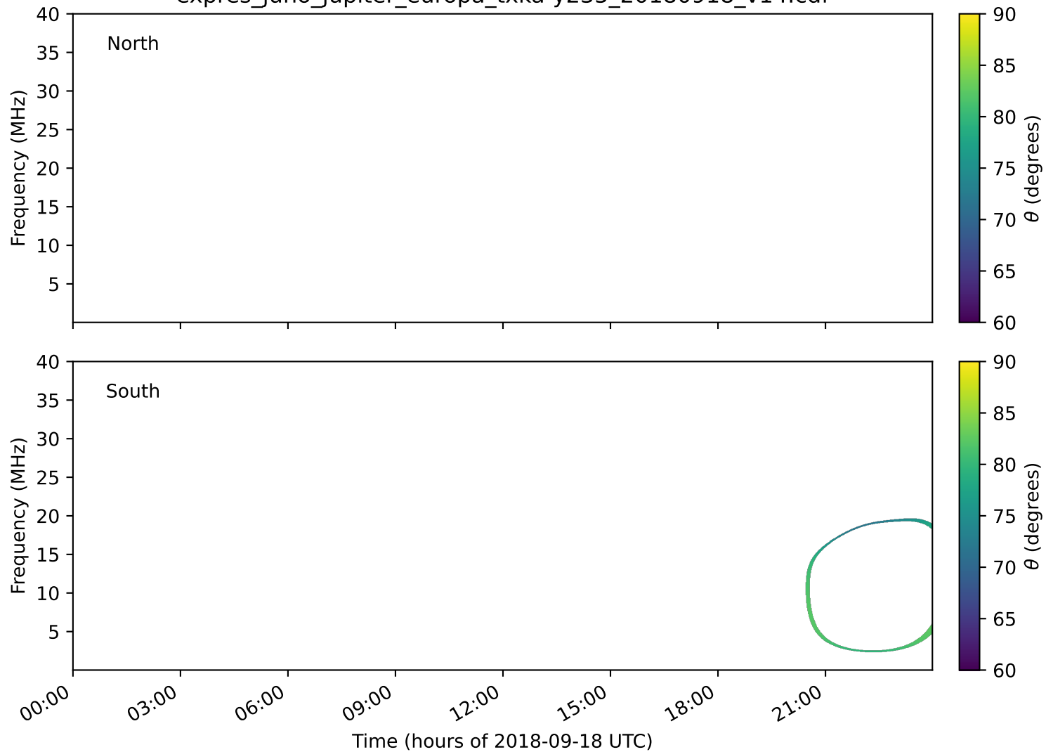
expres_juno_jupiter_europa_txka-y235_20180918_v14.cdf
