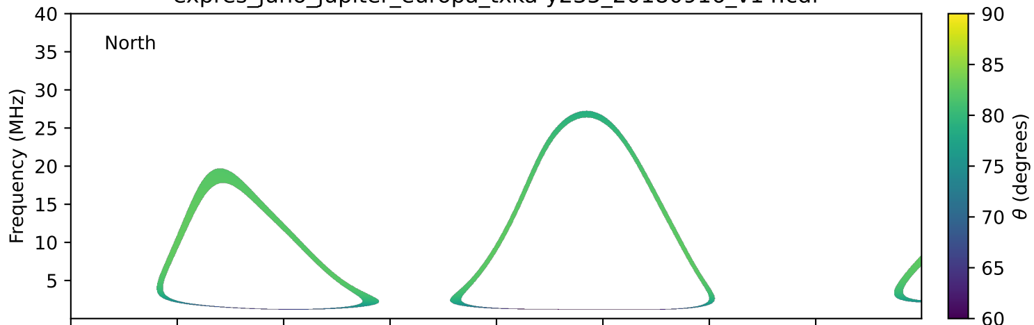
expres_juno_jupiter_europa_txka-y235_20180916_v14.cdf
