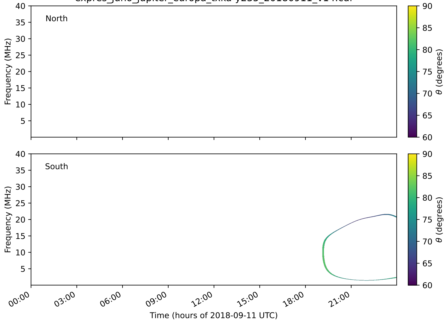
expres_juno_jupiter_europa_txka-y235_20180911_v14.cdf
