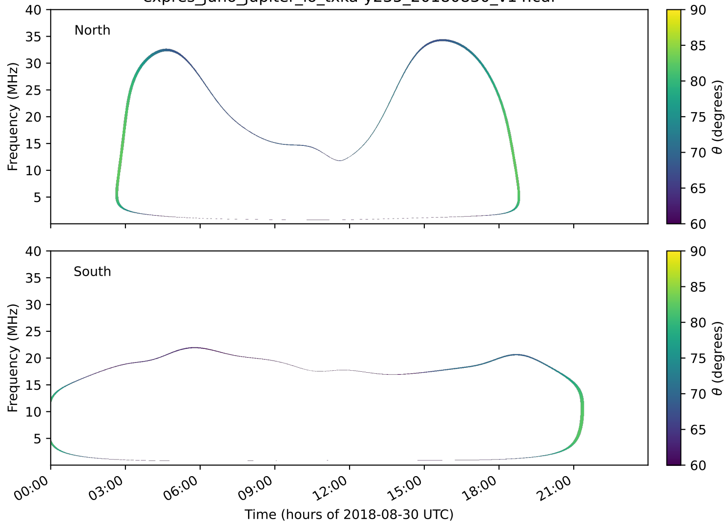
expres_juno_jupiter_io_txka-y235_20180830_v14.cdf
