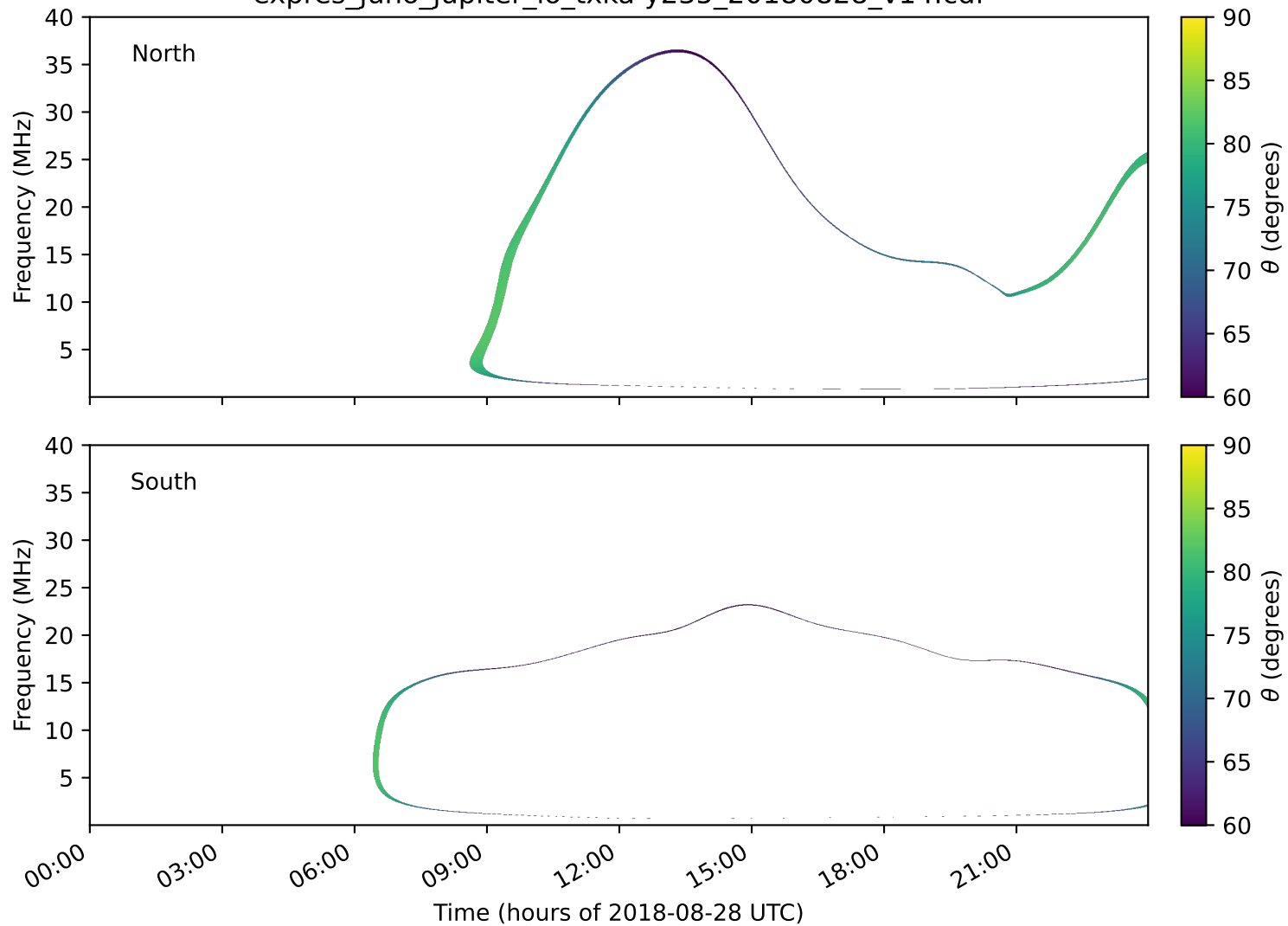
expres_juno_jupiter_io_txka-y235_20180828_v14.cdf
