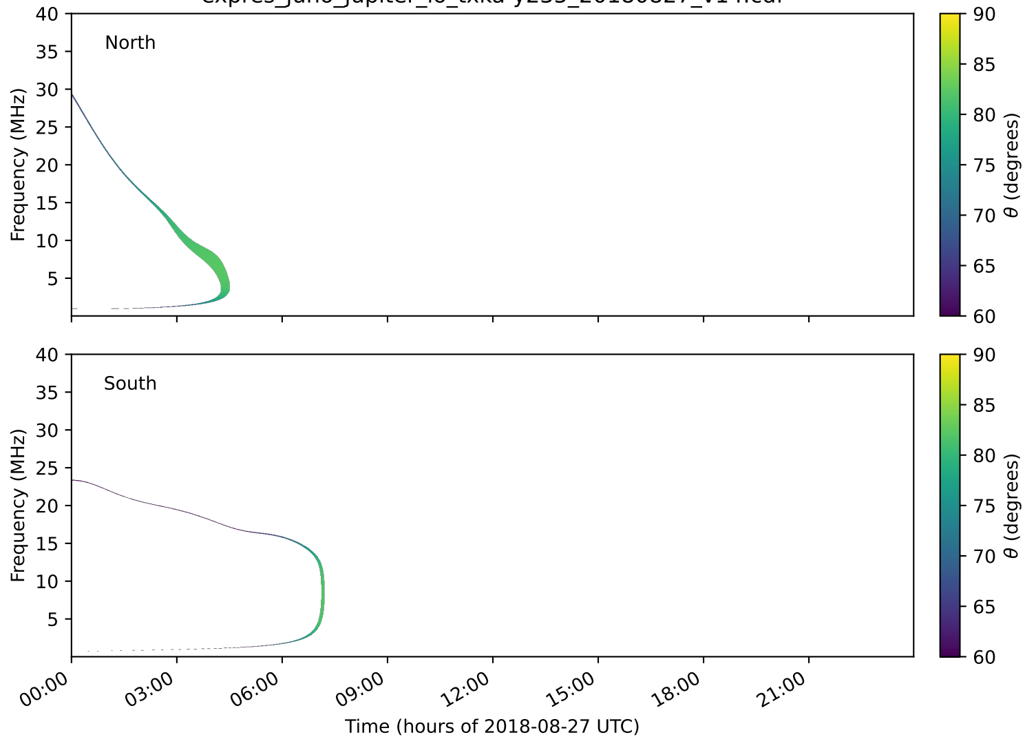
expres_juno_jupiter_io_txka-y235_20180827_v14.cdf
