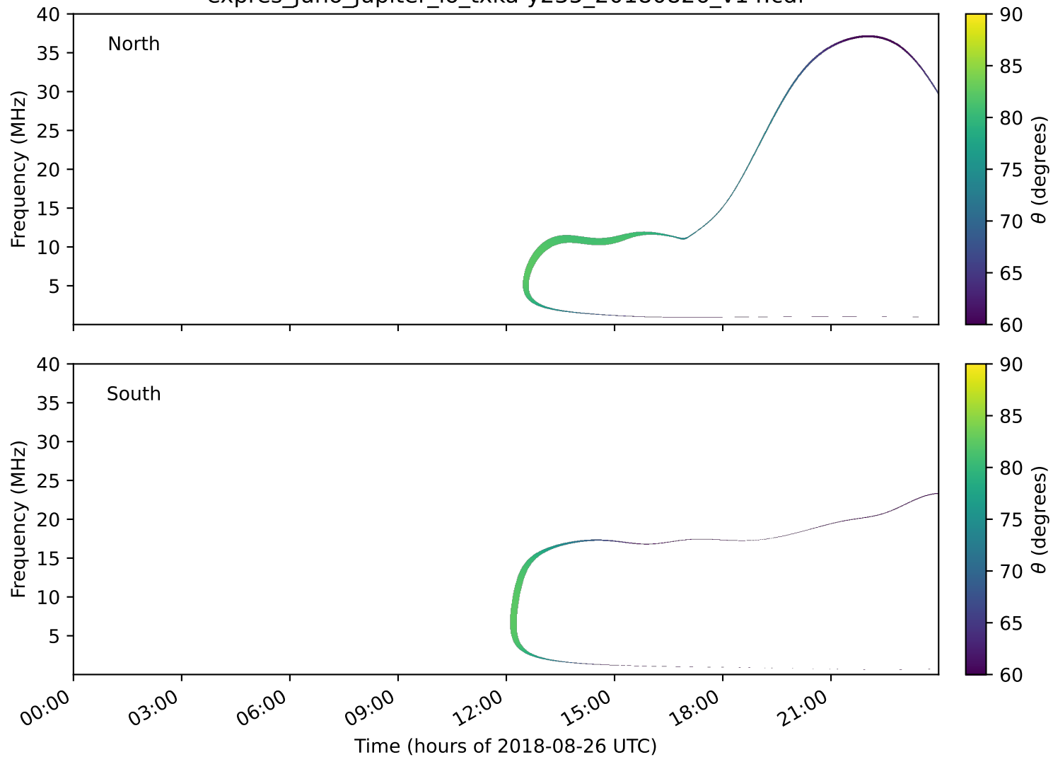
expres_juno_jupiter_io_txka-y235_20180826_v14.cdf
