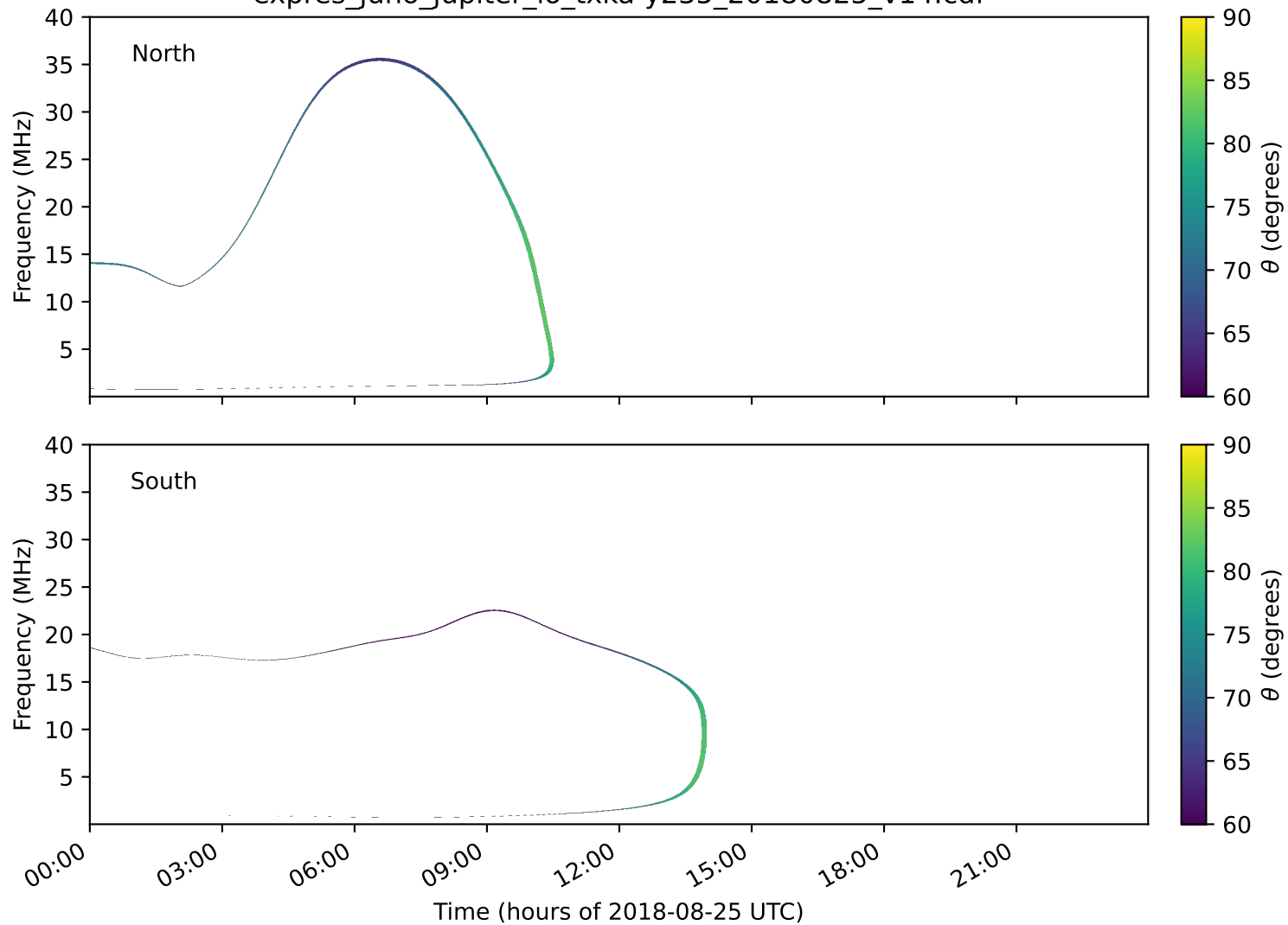
expres_juno_jupiter_io_txka-y235_20180825_v14.cdf
