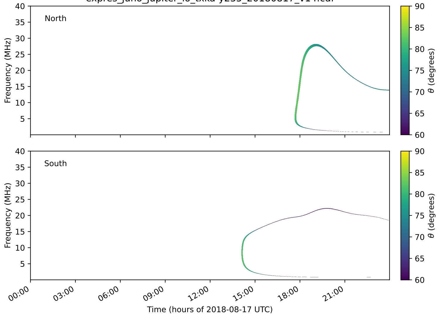
expres_juno_jupiter_io_txka-y235_20180817_v14.cdf
