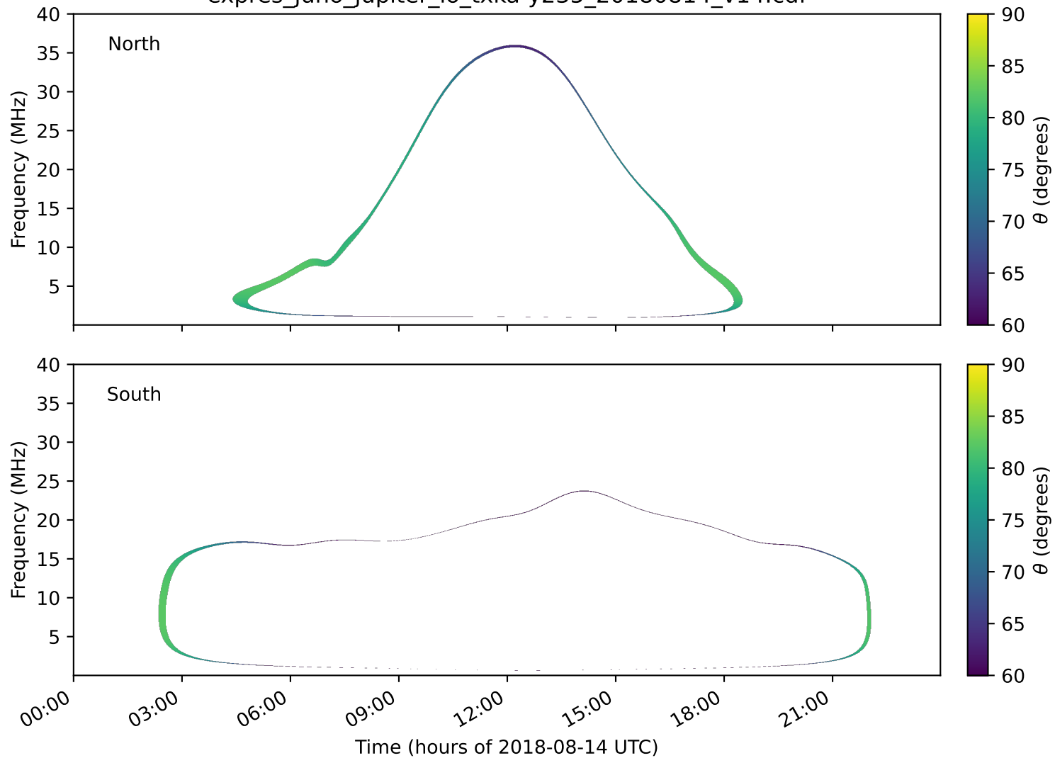
expres_juno_jupiter_io_txka-y235_20180814_v14.cdf
