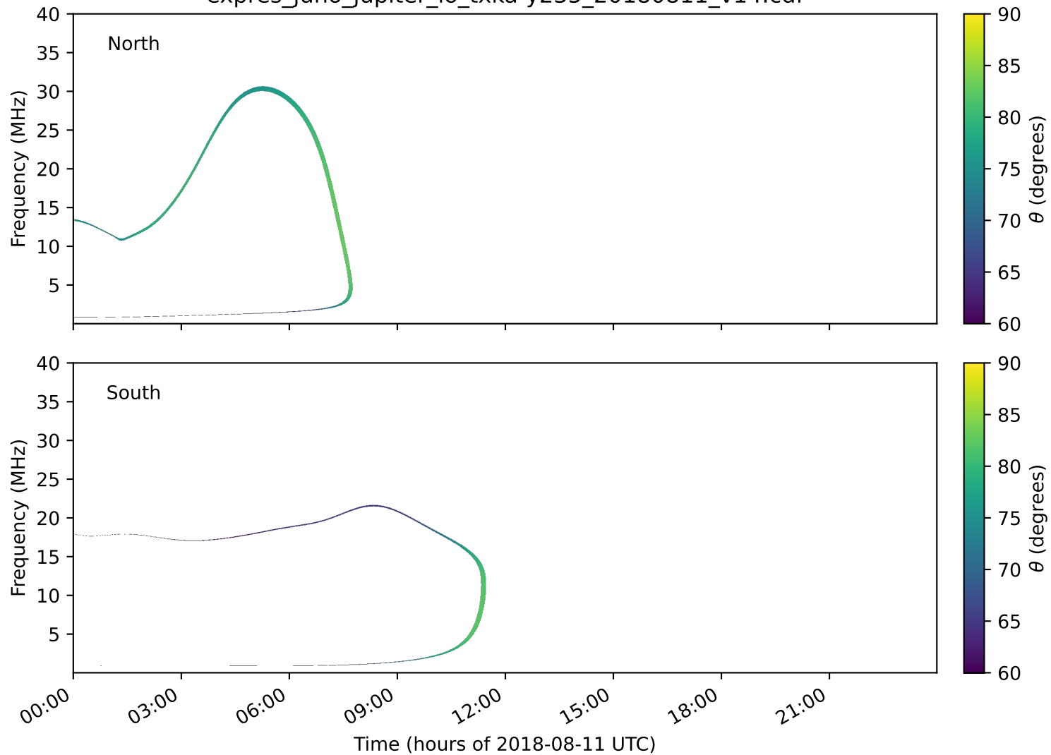
expres_juno_jupiter_io_txka-y235_20180811_v14.cdf
