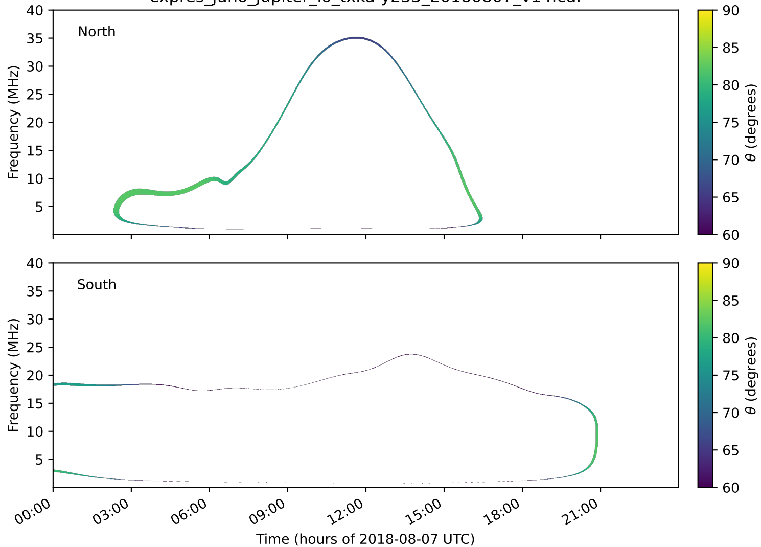
expres_juno_jupiter_io_txka-y235_20180807_v14.cdf
