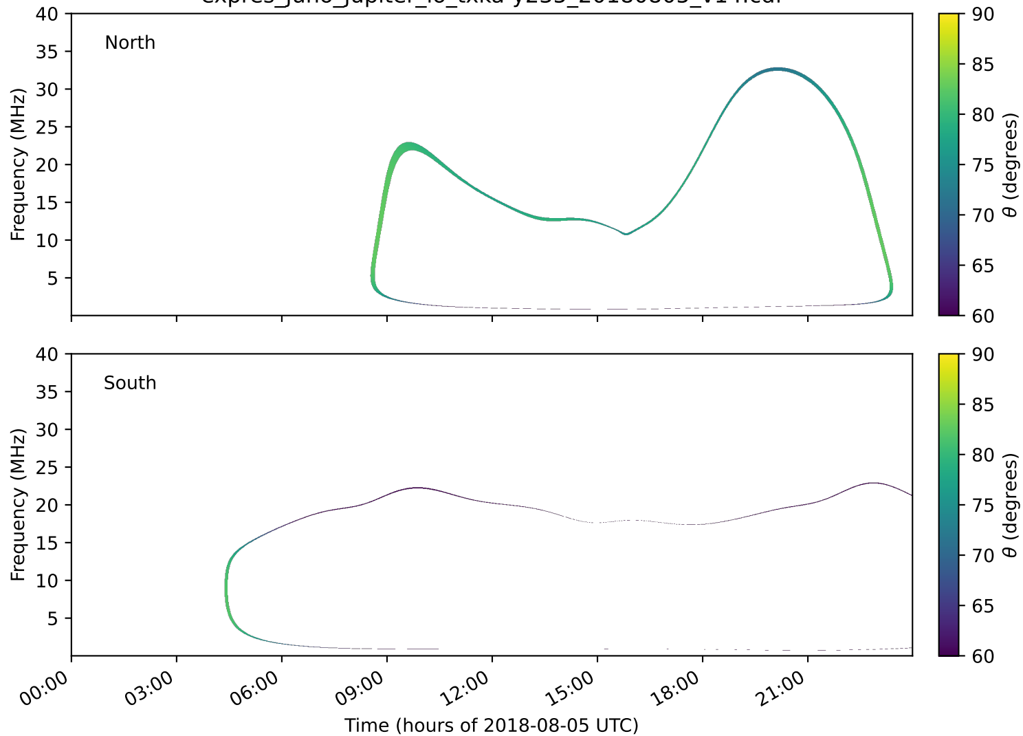
expres_juno_jupiter_io_txka-y235_20180805_v14.cdf
