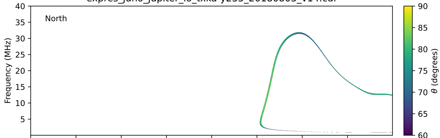
expres_juno_jupiter_io_txka-y235_20180803_v14.cdf
