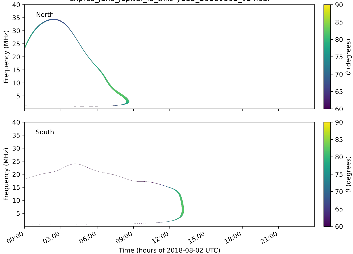
expres_juno_jupiter_io_txka-y235_20180802_v14.cdf
