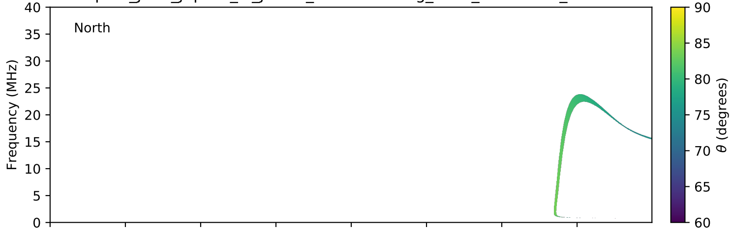
expres_juno_jupiter_io_jrm09_lossc-wid1deg_3kev_20180831_v01.cdf
