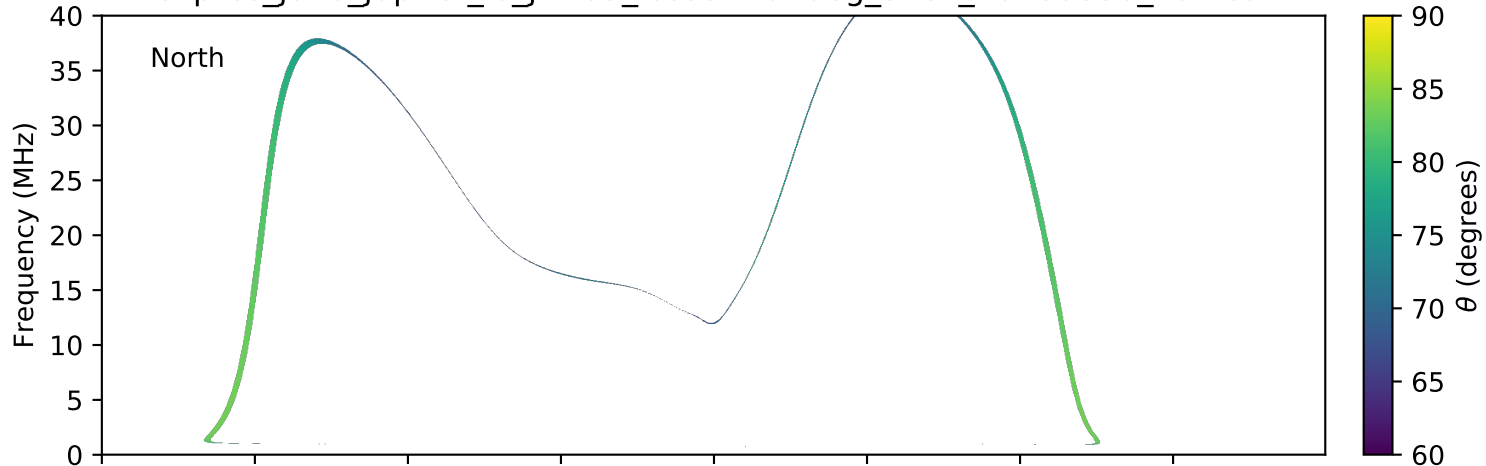
expres_juno_jupiter_io_jrm09_lossc-wid1deg_3kev_20180830_v01.cdf
