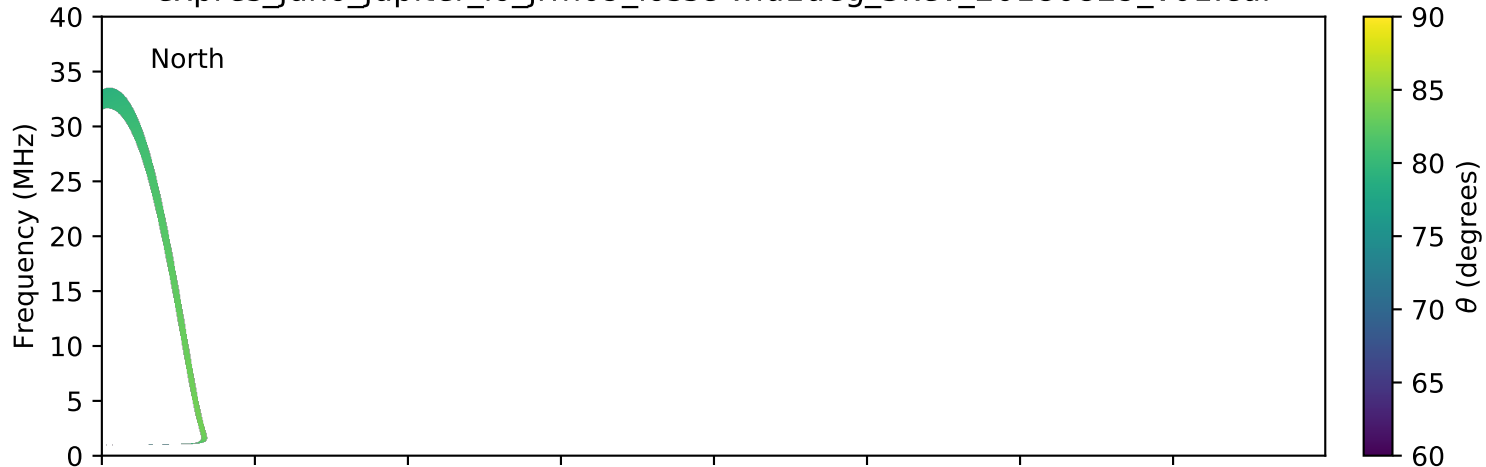
expres_juno_jupiter_io_jrm09_lossc-wid1deg_3kev_20180829_v01.cdf
