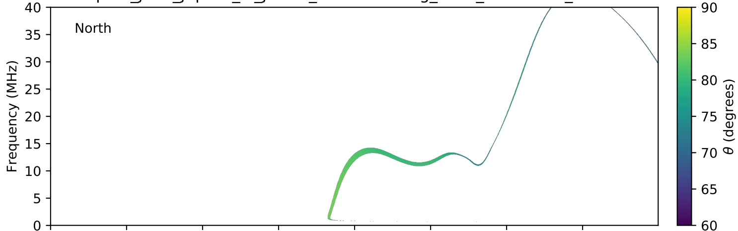
expres_juno_jupiter_io_jrm09_lossc-wid1deg_3kev_20180819_v01.cdf
