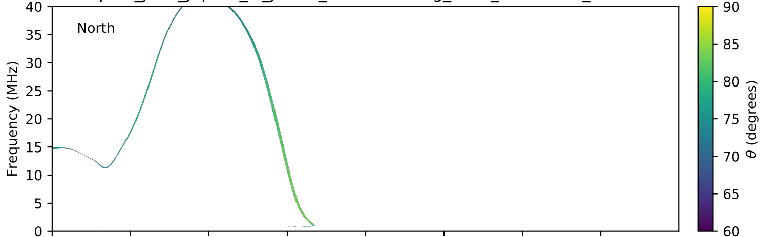
expres_juno_jupiter_io_jrm09_lossc-wid1deg_3kev_20180818_v01.cdf
