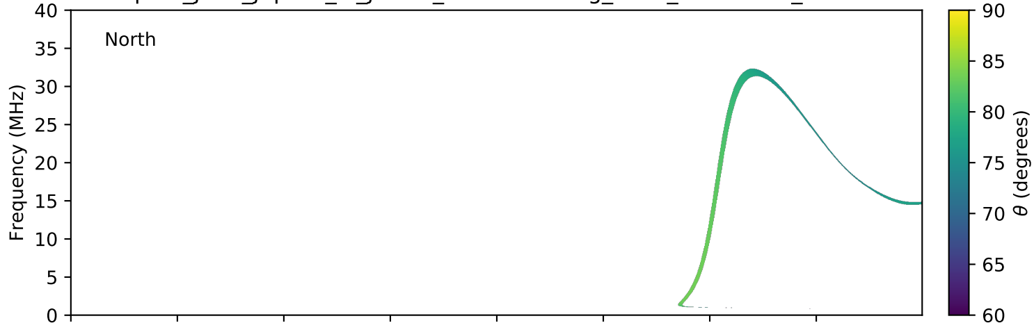
expres_juno_jupiter_io_jrm09_lossc-wid1deg_3kev_20180817_v01.cdf
