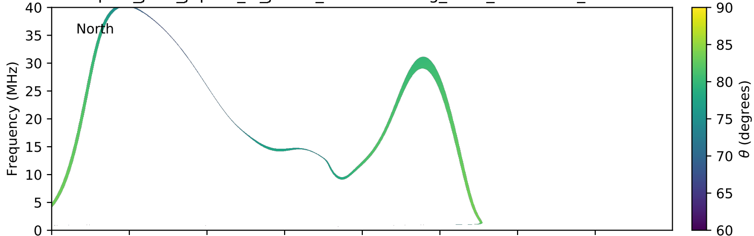
expres_juno_jupiter_io_jrm09_lossc-wid1deg_3kev_20180816_v01.cdf
