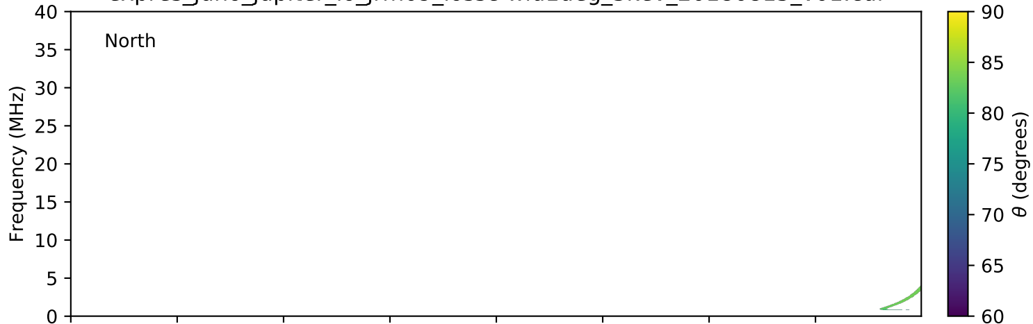
expres_juno_jupiter_io_jrm09_lossc-wid1deg_3kev_20180815_v01.cdf
