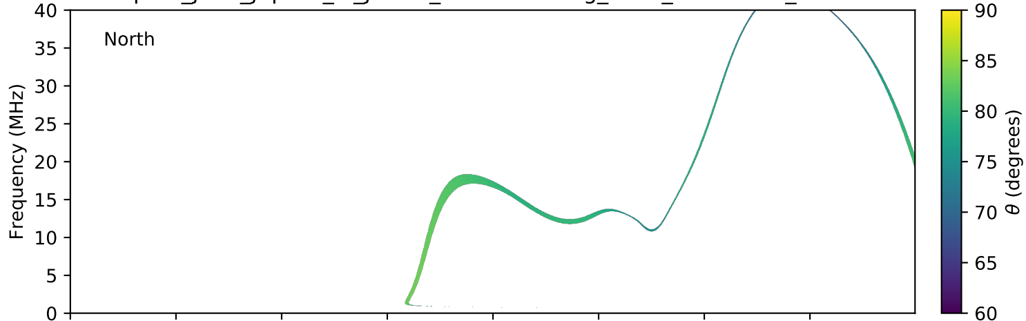
expres_juno_jupiter_io_jrm09_lossc-wid1deg_3kev_20180812_v01.cdf
