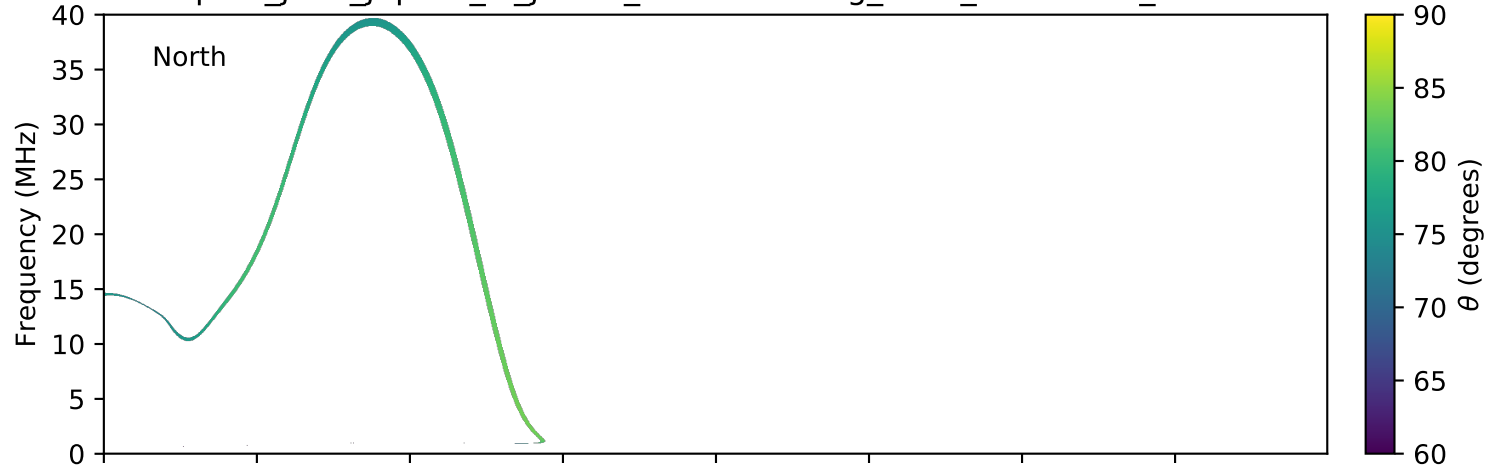
expres_juno_jupiter_io_jrm09_lossc-wid1deg_3kev_20180811_v01.cdf
