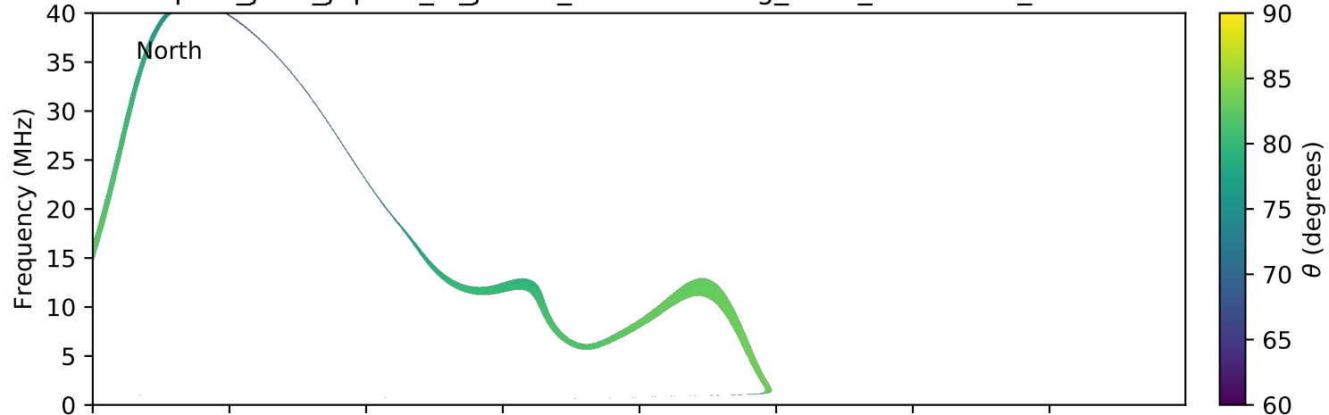
expres_juno_jupiter_io_jrm09_lossc-wid1deg_3kev_20180809_v01.cdf
