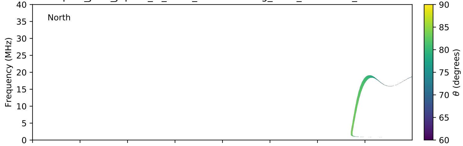
expres_juno_jupiter_io_isaac_lossc-wid1deg_3kev_20180831_v01.cdf
