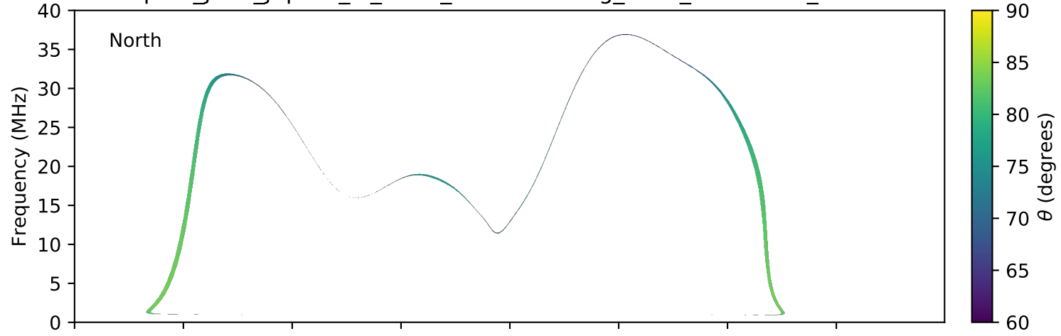
expres_juno_jupiter_io_isaac_lossc-wid1deg_3kev_20180830_v01.cdf
