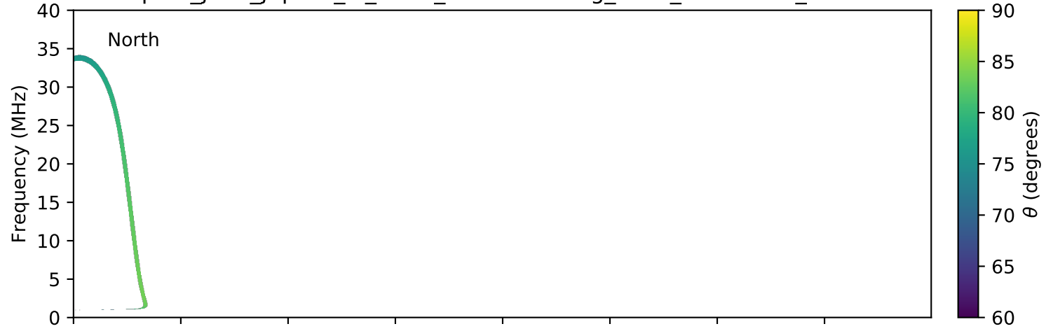
expres_juno_jupiter_io_isaac_lossc-wid1deg_3kev_20180829_v01.cdf
