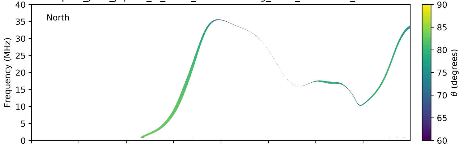
expres_juno_jupiter_io_isaac_lossc-wid1deg_3kev_20180828_v01.cdf
