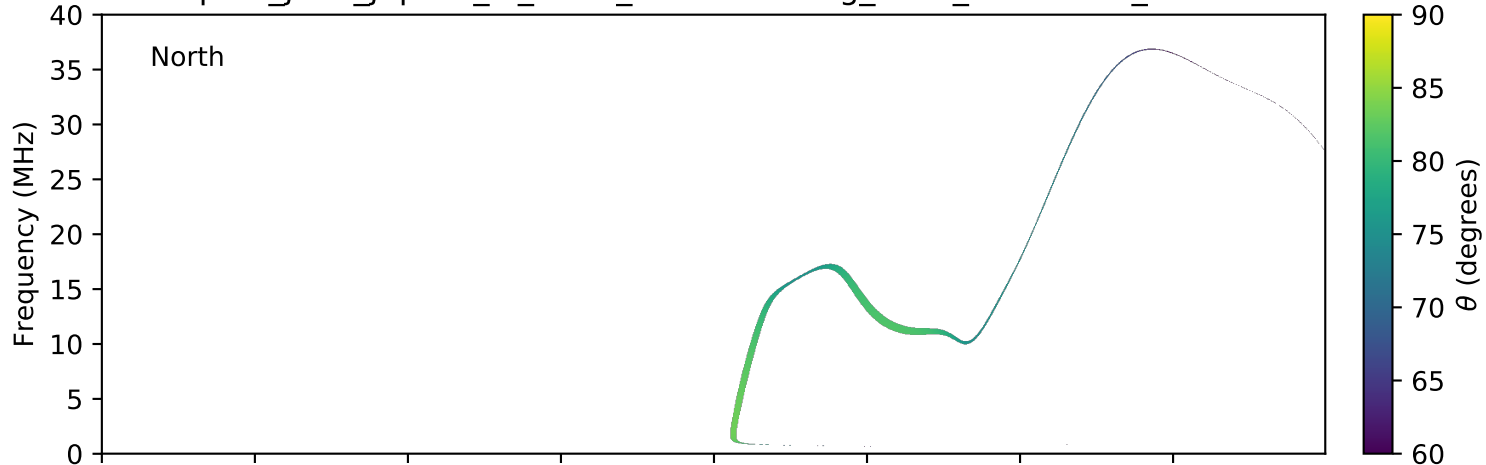
expres_juno_jupiter_io_isaac_lossc-wid1deg_3kev_20180826_v01.cdf
