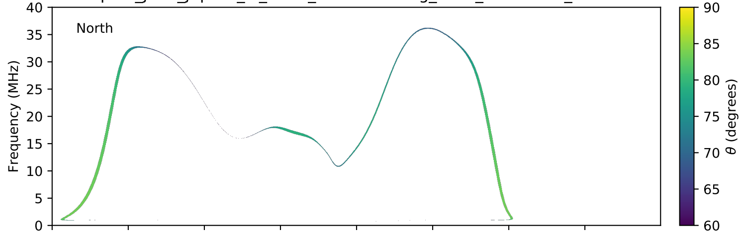
expres_juno_jupiter_io_isaac_lossc-wid1deg_3kev_20180823_v01.cdf
