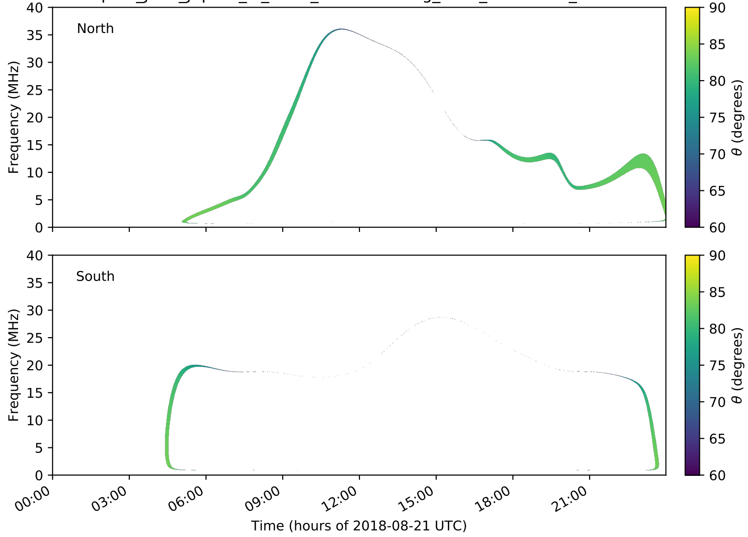
expres_juno_jupiter_io_isaac_lossc-wid1deg_3kev_20180821_v01.cdf
