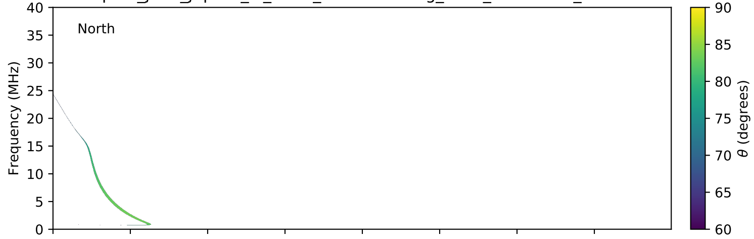
expres_juno_jupiter_io_isaac_lossc-wid1deg_3kev_20180820_v01.cdf
