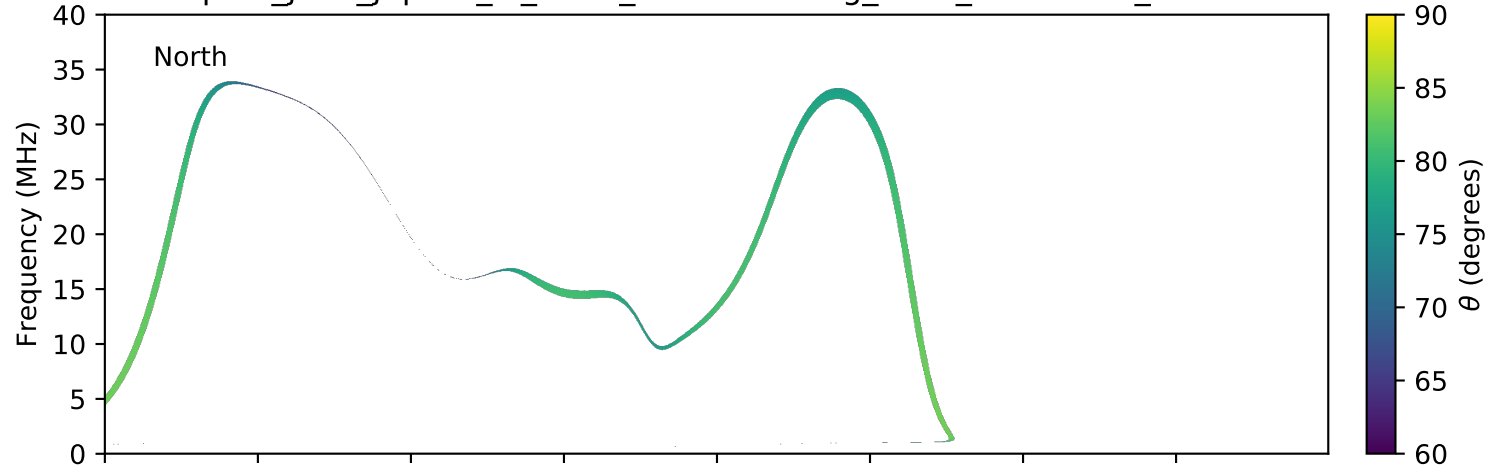
expres_juno_jupiter_io_isaac_lossc-wid1deg_3kev_20180816_v01.cdf
