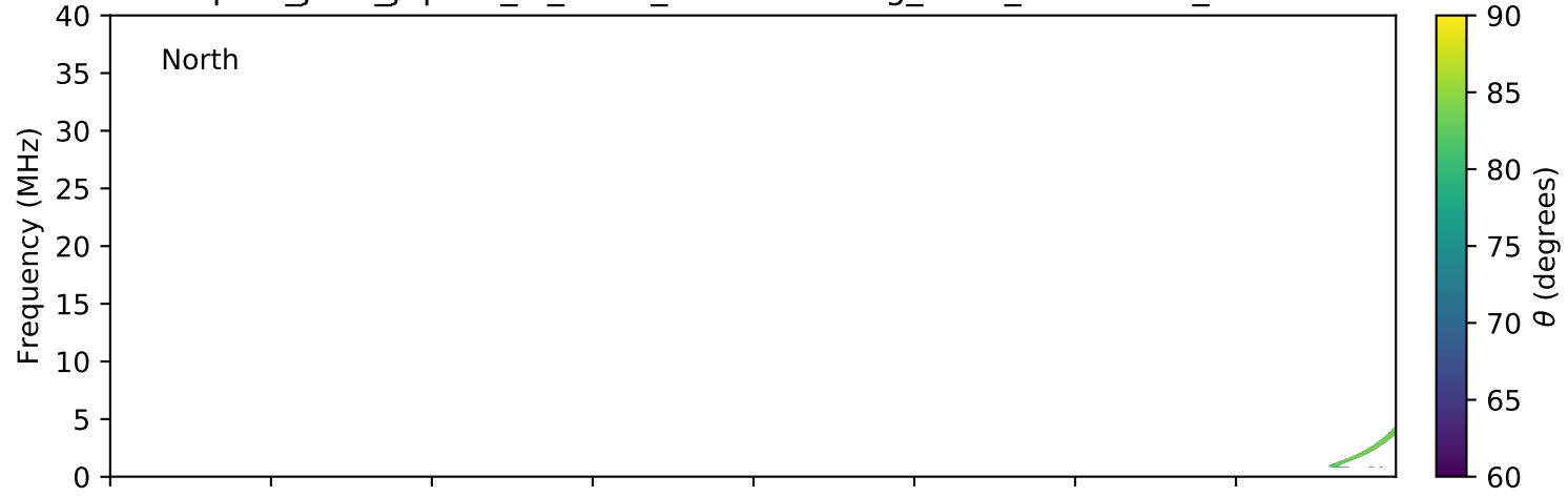
expres_juno_jupiter_io_isaac_lossc-wid1deg_3kev_20180815_v01.cdf
