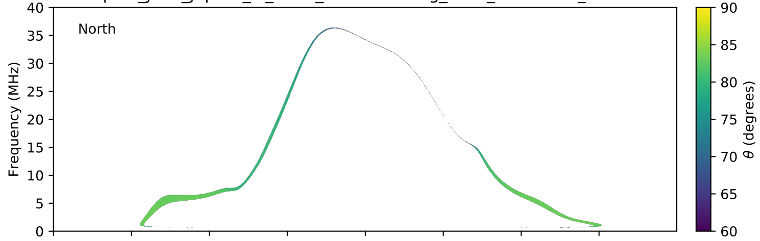
expres_juno_jupiter_io_isaac_lossc-wid1deg_3kev_20180814_v01.cdf
