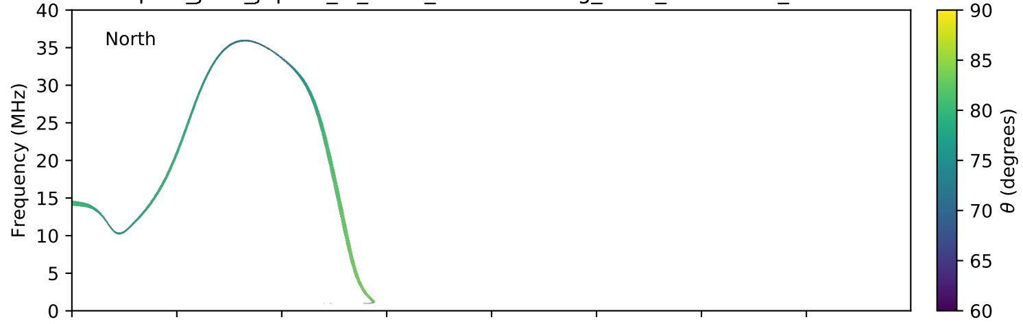
expres_juno_jupiter_io_isaac_lossc-wid1deg_3kev_20180811_v01.cdf
