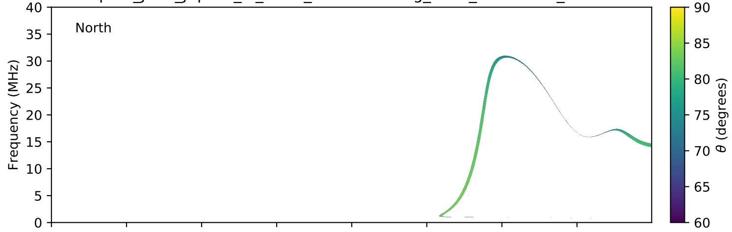
expres_juno_jupiter_io_isaac_lossc-wid1deg_3kev_20180810_v01.cdf
