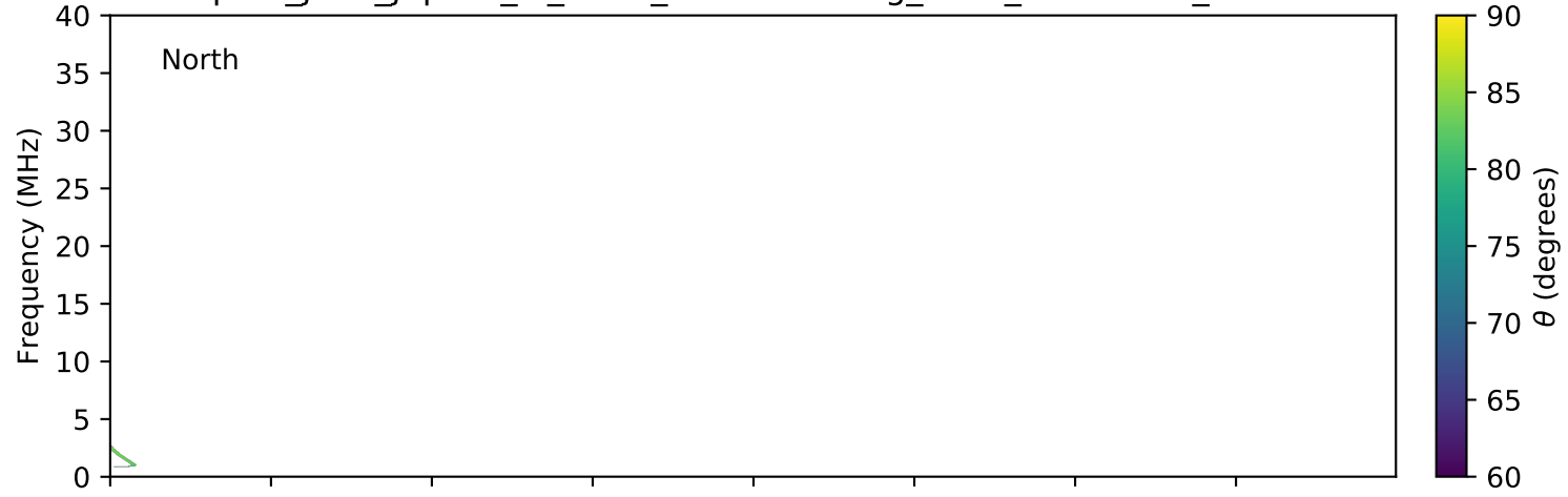
expres_juno_jupiter_io_isaac_lossc-wid1deg_3kev_20180806_v01.cdf
